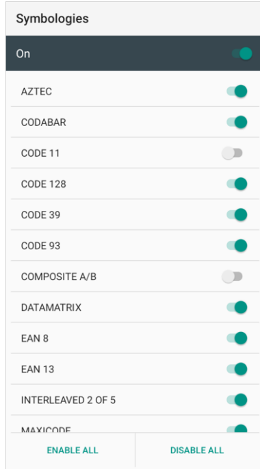
Figure 66 ScanSettings - Symbologies
