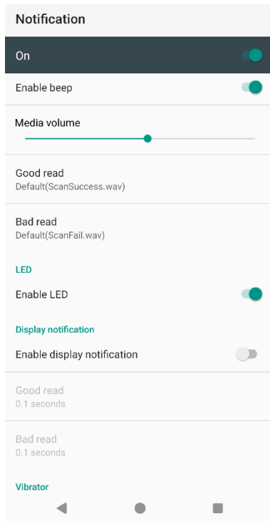
Figure 58 ScanSettings - Notification
