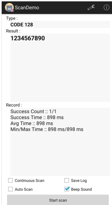
Figure 69 ScanDemo
