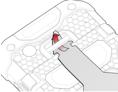
Figure 95 Mount hand strap_1
