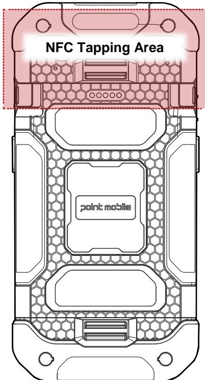
Figure 86 PM86 NFC tapping area
